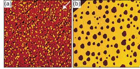
FIG. 14. (Color online) (Color online). (a) STM image after the adatom covered surface in Fig. 12(a) has been exposed to 0.5 MLE 5 keV Ar + at \vartheta = 83^\circ and 155 K. The arrow indicates the direction of the ion beam. Image size 850 \text{\AA} \times 850 \text{\AA} . (b) Same experiment as in (a) but after subsequent annealing to 720 K for 120 s. Image size 1750 \text{\AA} \times 1750 \text{\AA} .
