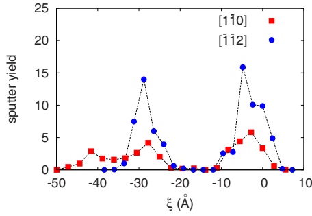
FIG. 7. (Color online) Azimuth dependence of sputtering. Sputter yield for ion incidence in [1\bar{1}0] and [\bar{1}\bar{1}2] azimuth onto a 7-island as a function of \xi for a stripe of width r_{NN} around \eta=0 , Eq. (9). Lines to guide the eyes.
