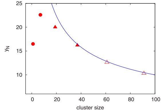
FIG. 6. (Color online) Sputter coefficient y_N vs island size N . Full circles: simulation results. Full triangles: Eq. (11), using simulation results for the sputter length X_{sp}(0) . Open triangles: Eq. (11), using X_{sp}(0) of the 37-island. Line: analytical law, Eq. (13), valid for N \geq 20 .
