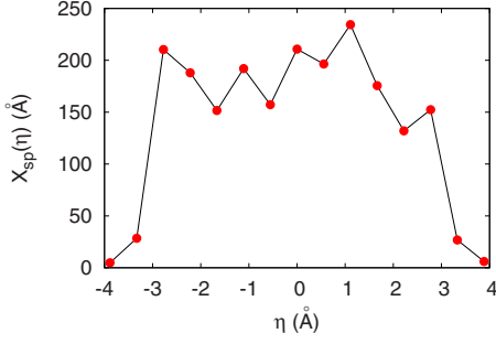
FIG. 3. (Color online) Dependence of sputter length X_{sp} on lateral position \eta of ion impact on 7-island. Lines to guide the eyes.
