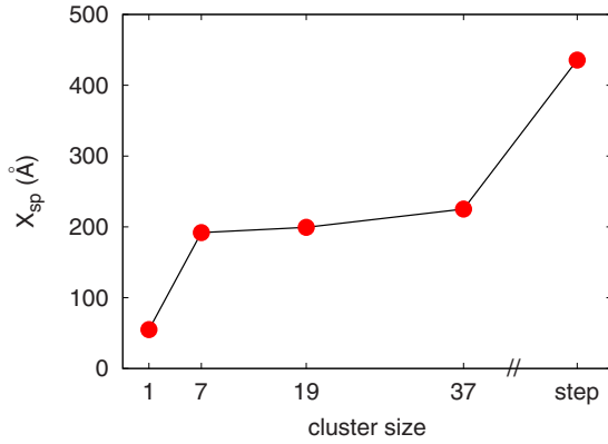
FIG. 5. (Color online) Dependence of the sputter length X_{sp}(0) on the island size N . Data calculated for \eta=0 . Lines to guide the eyes.
