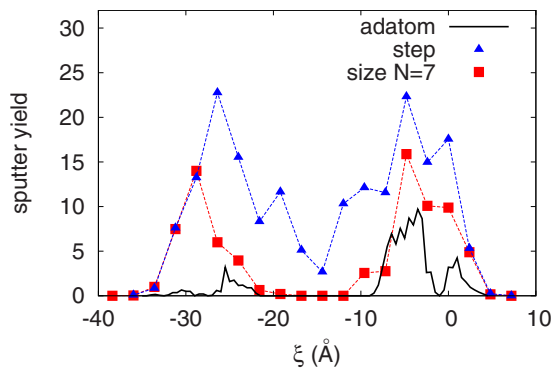
FIG. 4. (Color online) Dependence of the sputter yield on the distance \xi to the ascending island edge for central impacts, averaged over a stripe of width r_{NN} around \eta=0 , Eq. (9). Note that the data for the single adatom, N=1 , and for the step, N=\infty , are identical to the fully laterally averaged sputter yields. (a) Island size N=7, 19, 37 . (b) Island size N=1, 7, \infty . Lines to guide the eyes.
